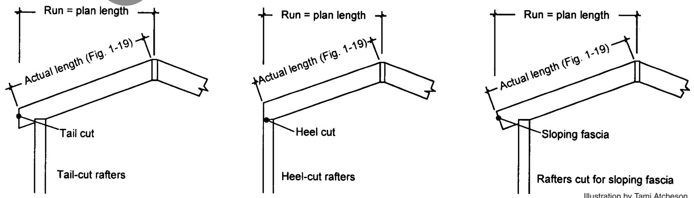
Figure 1-18 Run of various types of rafters
