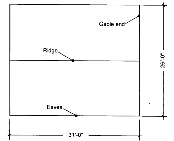
Figure 1-22 Gable roof example
