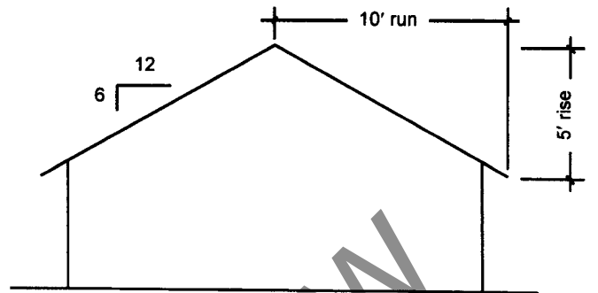
Figure 1-9 Roof rise and run
