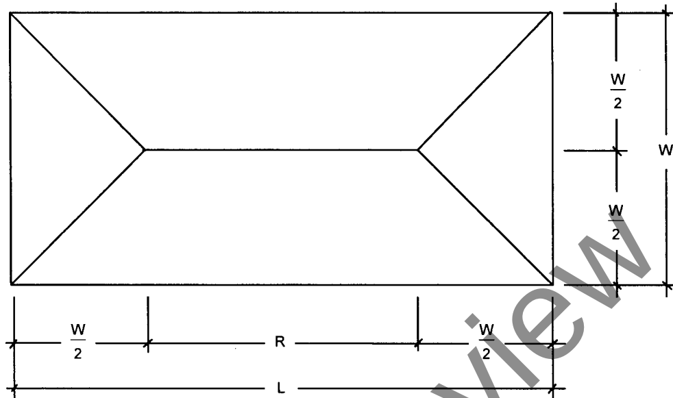
Figure 1-28 Ridge length
