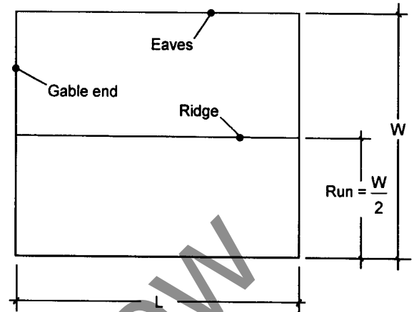
Figure 1-17 Plan view of gable roof
