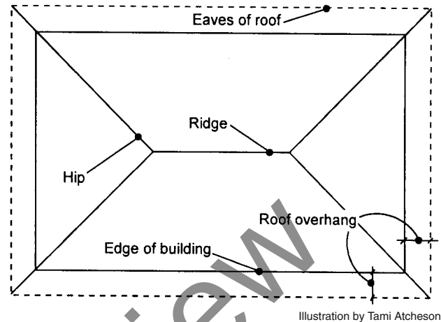
Figure 1-25 Roof overhangs
